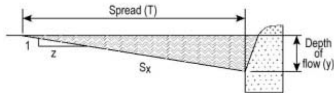
Figure ST-1 — Typical Gutter Section – Constant Cross Slope (VDOT Drainage Manual 2010)
